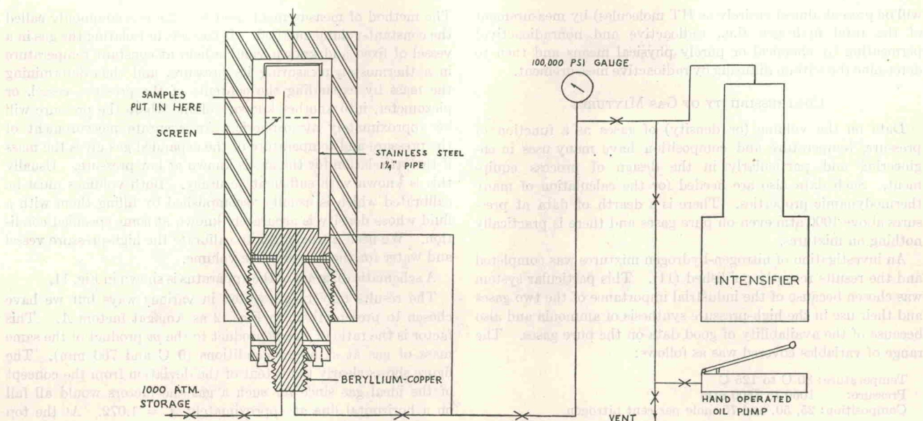
FIG. 10 DIAGRAM OF APPARATUS FOR TESTS OF HYDROGEN EMBRITTLEMENT AT ROOM TEMPERATURE
