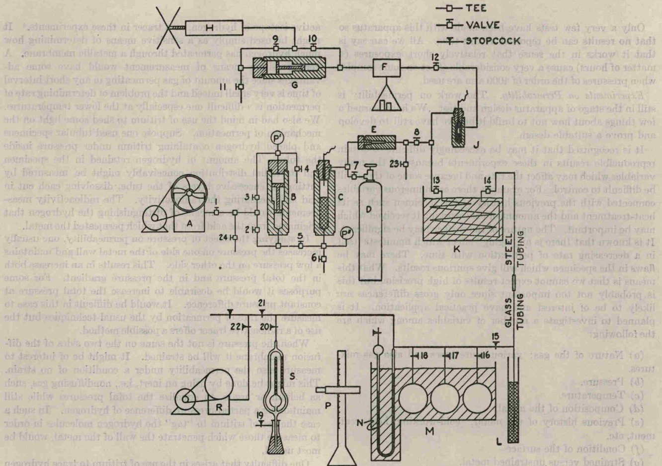
FIG. 11 DIAGRAM OF APPARATUS FOR COMPRESSIBILITY MEASUREMENT
